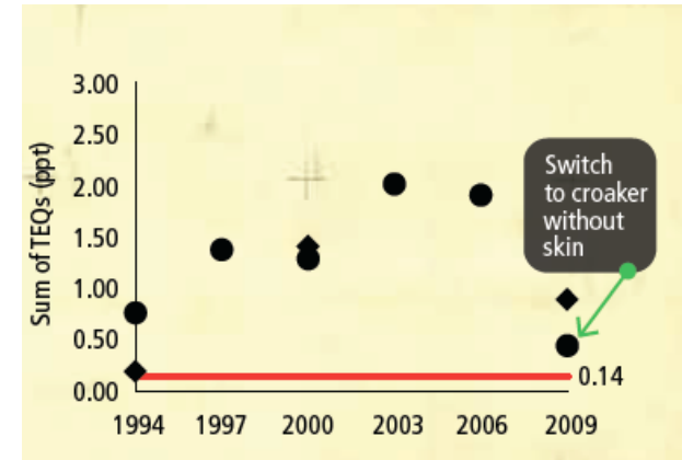
Dioxin and furan TEQ concentrations (ppt) in white croaker (circles) and shiner surfperch (diamonds). Baywide averages.
