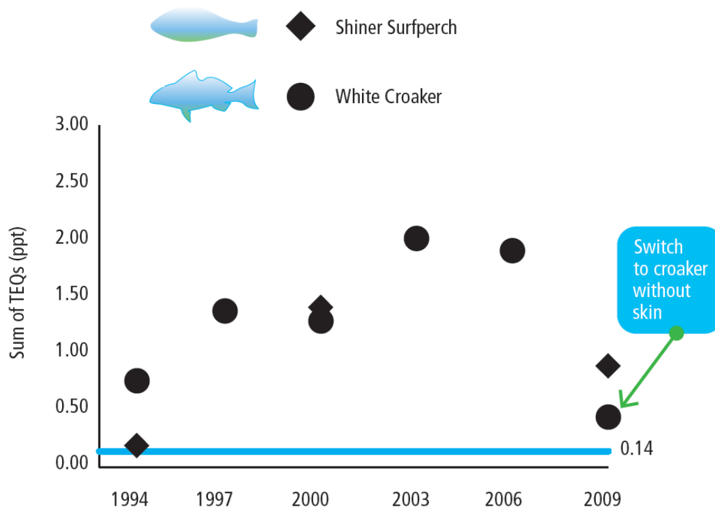
Baywide average dioxin and furan TEQ concentrations (ppt) in white croaker (circles) and shiner surfperch (diamonds). Blue line indicates screening value.
